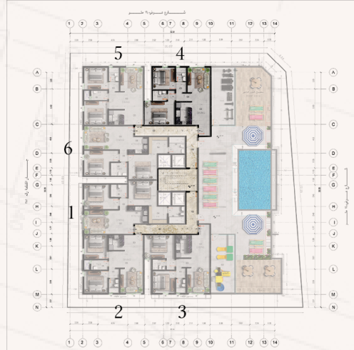
Apartment 4 North-facing Total area: 93.72 m 2
